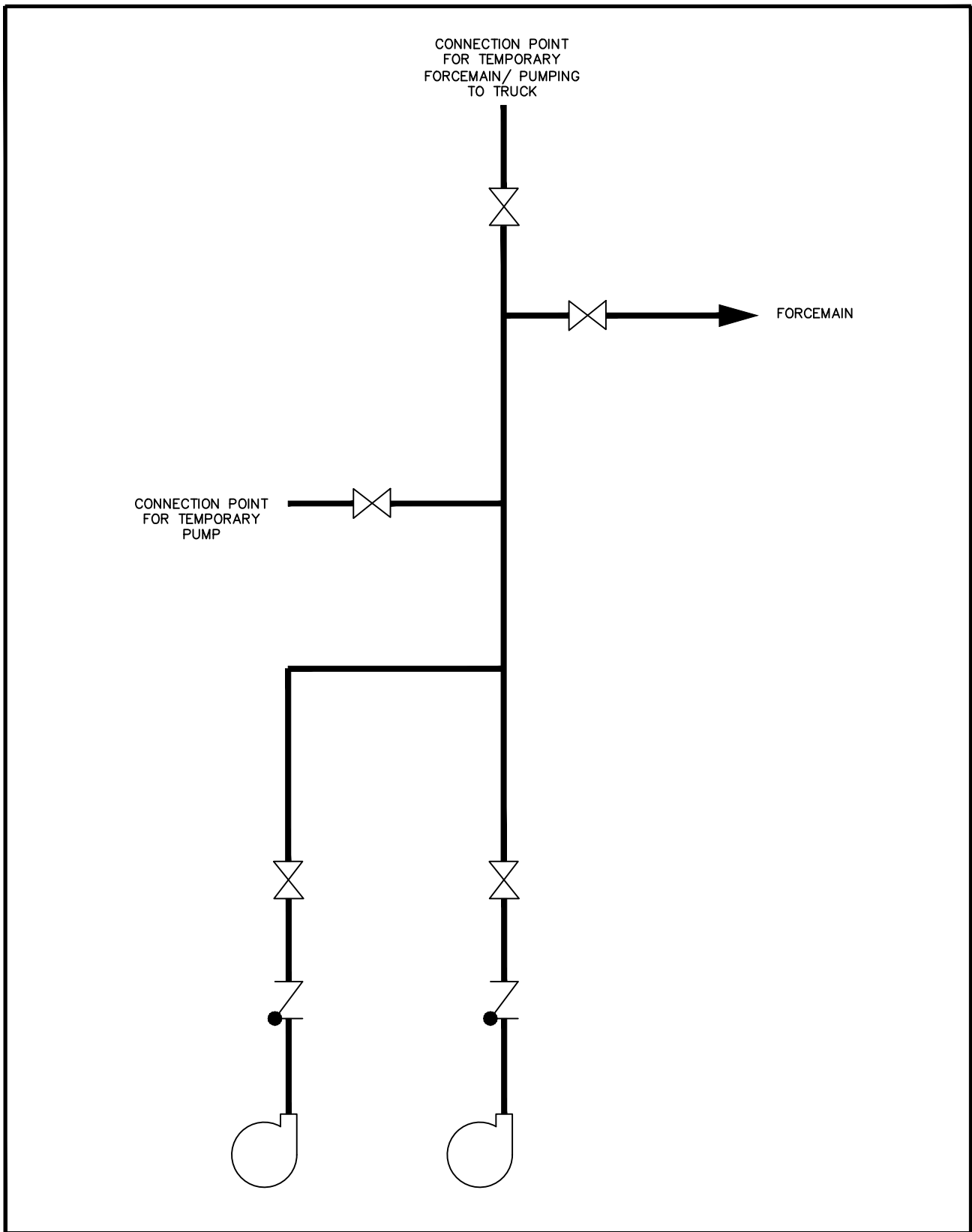
FIGURE 6-2 PIPING BYPASS ARRANGEMENT (DESIGN I AND II)
