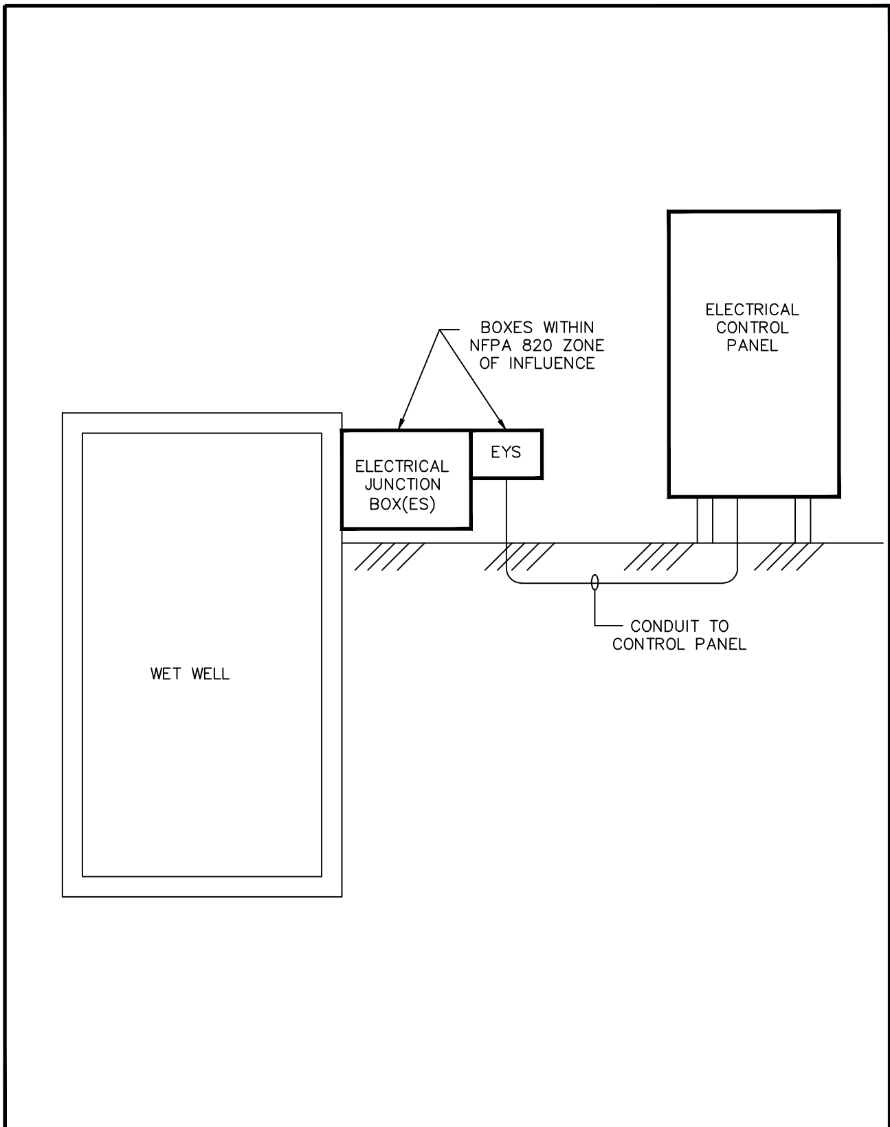
FIGURE 6-3 ELECTRICAL BOX LOCATIONS
